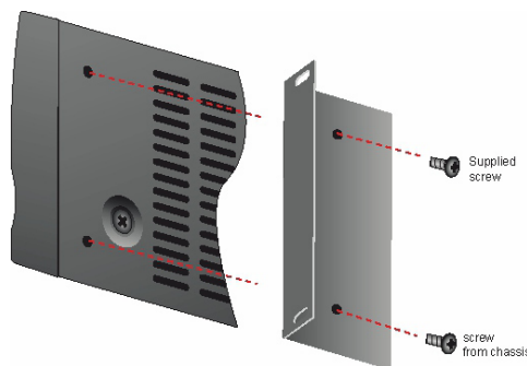
[Figure 2.1 Comment installer les supports de rack]
